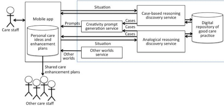
Figure 1 The Carer architecture, showing how digital sharing of knowledge about good practices related to care is used by computational creativity services to deliver support to care staff (see online version for colours)
