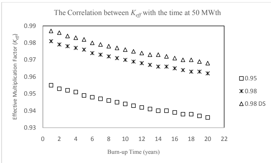
Figure 13 The effective multiplication factor ( K_{eff} ) for a duration of 20 years of balance type reactor at 50 MW-th power output at K_{eff} 0.95, 0.98 and 0.98 DS
