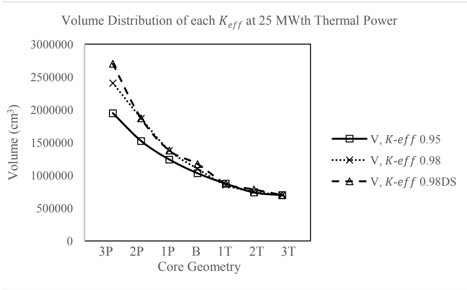
Figure 8 The correlation between volume distribution with the core geometry at all simulated K_{eff} value at 25 MW-th power output
