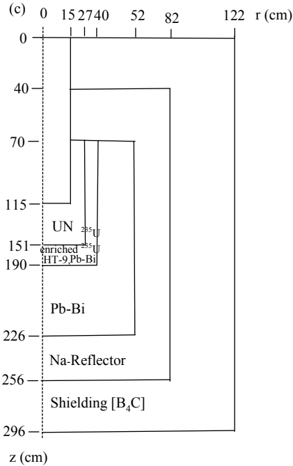
Figure 11 Comparison of half cross-sectional view of core geometry at 50 MW-th power output between (a) K_{eff} 0.95 (b) K_{eff} 0.98 and (c) K_{eff} 0.98 DS (continued)
