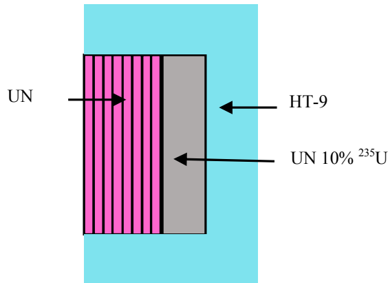
Figure 1 Presents the vertical cross-section of a tall type 3× (3T) at 10 MW-th power output at a K_{eff} value of 0.98. Half of a cross-sectional view is displayed
