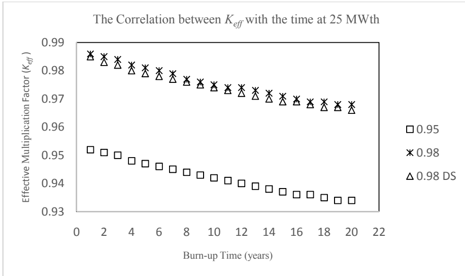
Figure 9 The effective multiplication factor ( K_{eff} ) for a duration of 20 years of balance type reactor at 25 MW-th power output at K_{eff} 0.95, 0.98 and 0.98 DS
