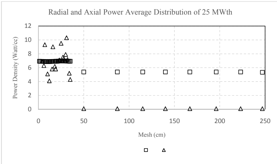
Figure 10 Average distribution of radial and axial at 25 MW-th power output
