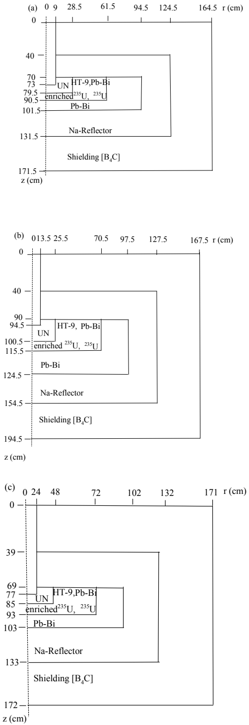
Figure 3 Comparison of half cross-sectional view of core geometry at 10 MW-th power output between (a) K_{eff} 0.95 (b) K_{eff} 0.98 and (c) K_{eff} 0.98 DS
