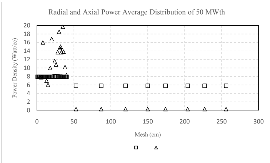
Figure 14 Average distribution at radial and axial at 50 MW-th power output
