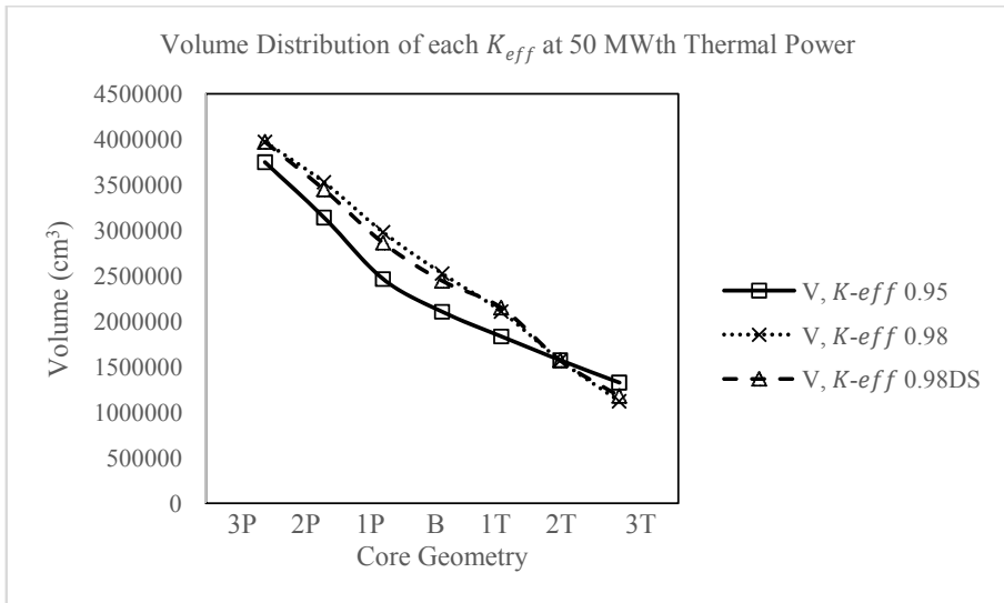
Figure 12 The correlation between volume distribution with the core geometry at all simulated K_{eff} value at 50 MW-th power output
