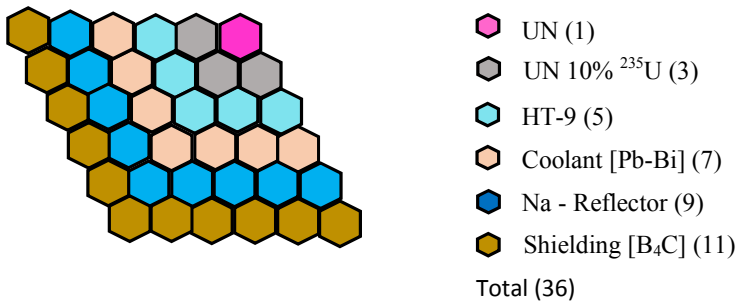
Figure 2 Illustrates the horizontal cross-section of a tall type 3× (3T) at 10 MW-th power output at a K_{eff} value of 0.98. A quarter of a cross-sectional view is displayed (see online version for colours)
