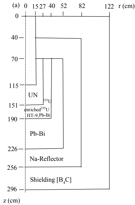
Figure 11 Comparison of half cross-sectional view of core geometry at 50 MW-th power output between (a) K_{eff} 0.95 (b) K_{eff} 0.98 and (c) K_{eff} 0.98 DS
