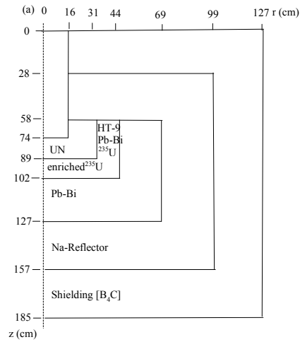
Figure 7 Comparison of half cross-sectional view of core geometry at 25 MW-th power output between (a) K_{eff} 0.95 (b) K_{eff} 0.98 and (c) K_{eff} 0.98 DS
