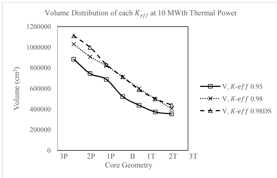
Figure 4 The correlation between volume distribution with the core geometry at all simulated K_{eff} value at 10 MW-th power output
