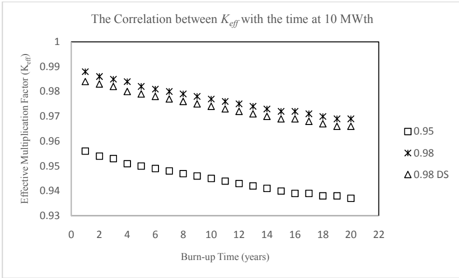
Figure 5 The effective multiplication factor ( K_{eff} ) for a duration of 20 years of balance type reactor at 10 MW-th power output at K_{eff} 0.95, 0.98 and 0.98 DS
