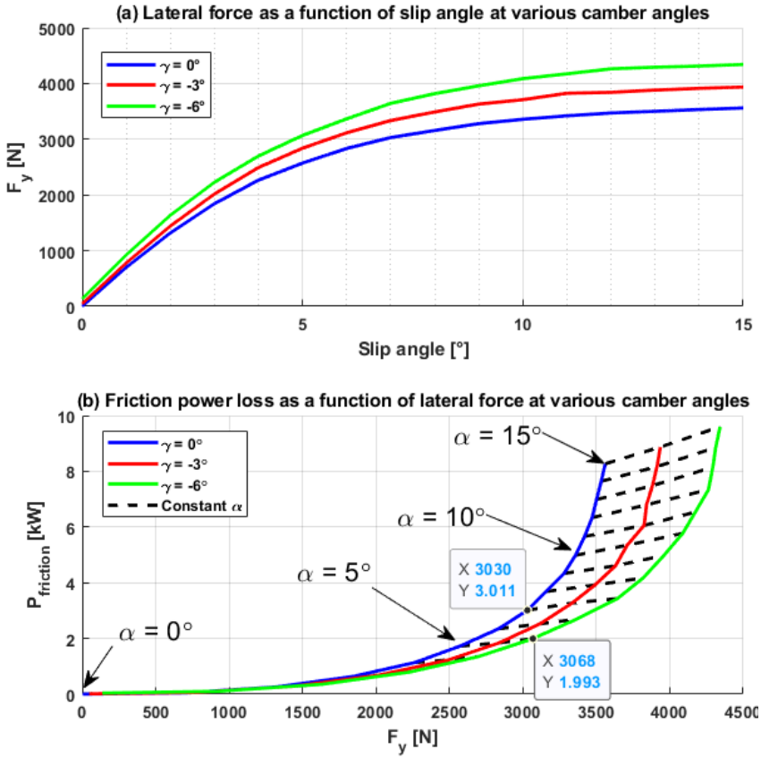
Figure 3 (a) Lateral force vs. slip angle for three camber angles at a vertical load of 3500 N and (b) friction power loss as a function of lateral force at various camber angles at a vertical load of 3500 N (see online version for colours)
