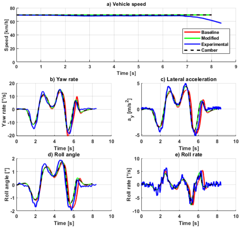
Figure 5 Comparison of severe double lane change simulation results for baseline, modified baseline and camber models with experimental data gathered on test vehicle in baseline configuration (see online version for colours)
