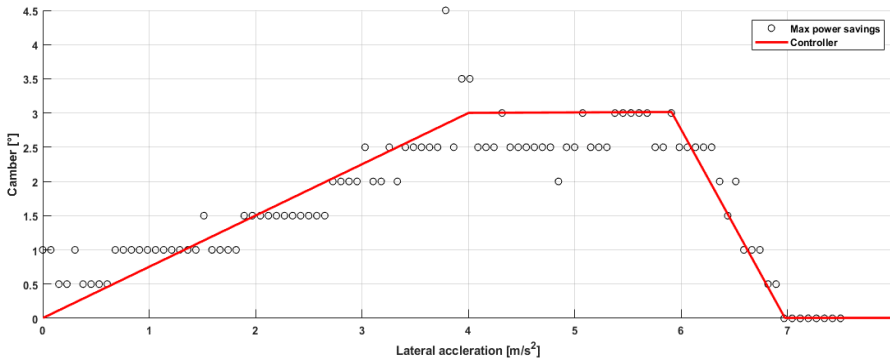
Figure 8 Maximum power savings derived from Figure 7(a) and proposed camber angle setpoint (see online version for colours)
