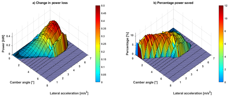
Figure 7 (a) Change in power loss during constant radius tests and(b) percentage power saved during constant radius tests (see online version for colours)
