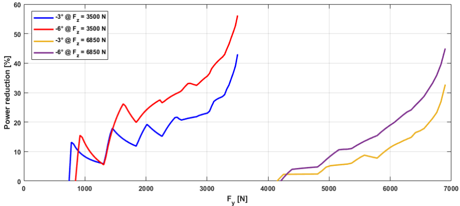
Figure 4 Power reduction possible by adding camber angle to slip angle at various tyre lateral forces and vertical tyre loads (image cropped to indicate power savings) (see online version for colours)
