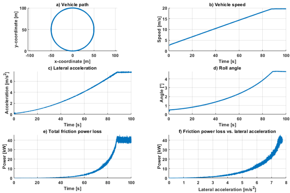
Figure 6 Constant radius test simulation results at -4^\circ camber (see online version for colours)
