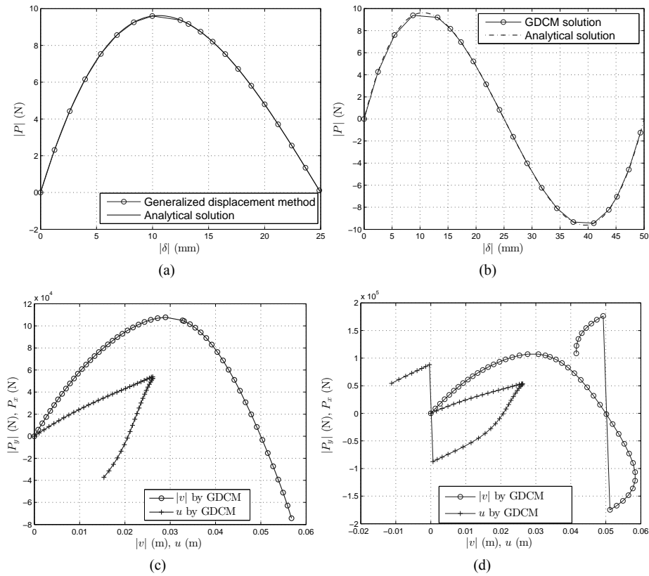
Figure 2 2D co-rotational truss solution by GDCM approach, (a) snap through (b) snap back behaviour, 2D truss configuration as shown in Figure 1(b) solved by GDCM with inputs as (c) (P_x)_4 = 4 \times 10^3 , (P_y)_4 = -8 \times 10^3 , and \lambda_1^1 = 0.75 (d) (P_x)_4 = 6 \times 10^3 , (P_y)_4 = -12 \times 10^3 , and \lambda_1^1 = 0.75
