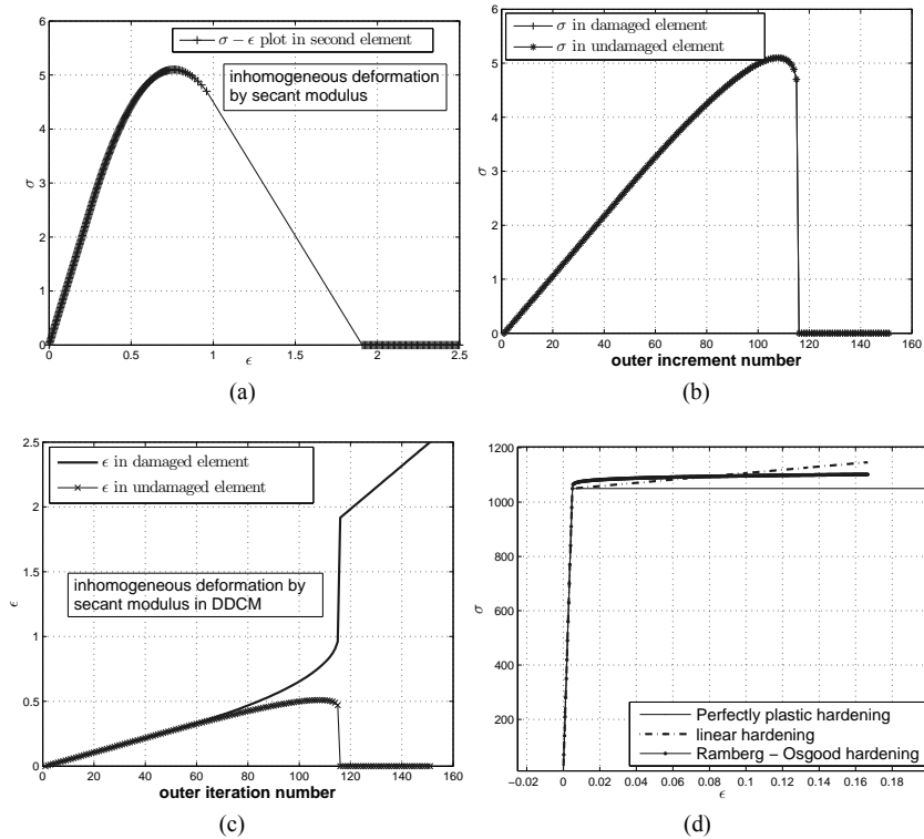
Figure 7 1D bar under uniaxial tension solved by ID and E = K_s , (a) \sigma - \epsilon plot within damaged element (b) variation of \sigma within undamaged and damaged elements (c) variation of \epsilon within damaged and undamaged elements (d) HD case solved by return-mapping plasticity algorithms
