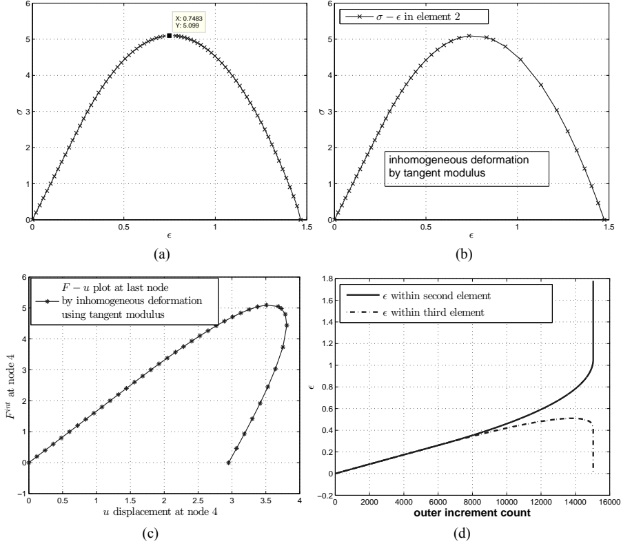
Figure 3 \sigma vs. \epsilon plot in 1D bar under uniaxial tension solved by GDCM considering E = E_T , (a) HD (b) ID cases, 1D bar under uniaxial tension (c) F^{int} - u at last node with ID case and E = E_T (d) strain variation in damaged element (2nd) and last element obtained by ID case and E = K_s
