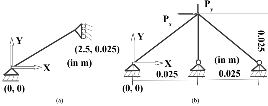
Figure 1 (a) One bar truss (b) Three bar truss configurations
