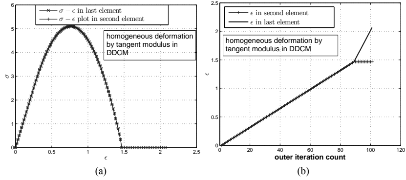
Figure 6 1D bar under uniaxial tension solved by DDCM for HD case and E = E_T , (a) \sigma - \epsilon plot in second and last elements (b) variation in \epsilon in last and second (interior) element
