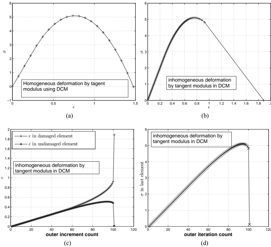
Figure 5 1D bar under uniaxial tension solved by DCM using E = E_T , (a) \sigma - \epsilon plot for HD (b) \sigma - \epsilon plot for ID case (within damaged element) (c) \epsilon variation in damaged and undamaged elements (d) \sigma within undamaged element (last) for ID case
