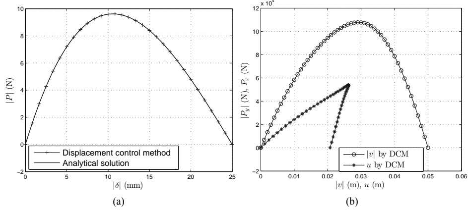
Figure 4 (a) Load vs. displacement in Y -direction at node 2 for 2D truss configuration, as shown in Figure 1(a), solved by DCM (b) Load vs. displacement in X - and Y -directions at node 4 in 2D truss configuration, as shown in Figure 1(b), solved by DCM
