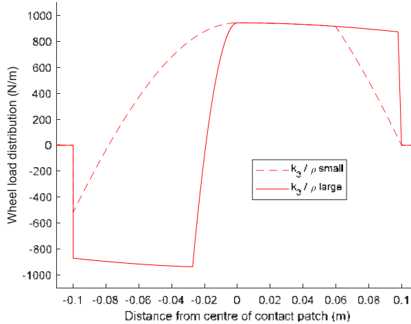
Figure 10 Wheel load from Masing model, for a rolling tyre (see online version for colours)
