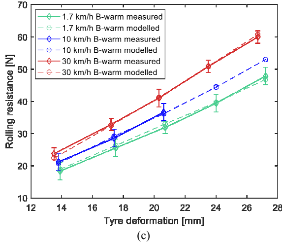
Figure 7 The measured and modelled rolling resistance against deformation for the three studied cases. The error bars indicate the measurement uncertainties: (a) cold class A tyre; (b) cold class B tyre and (c) warm class B tyre (see online version for colours) (continued)
