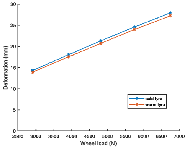
Figure 5 Tyre deformation for class B tyre (static measurement) (see online version for colours)
