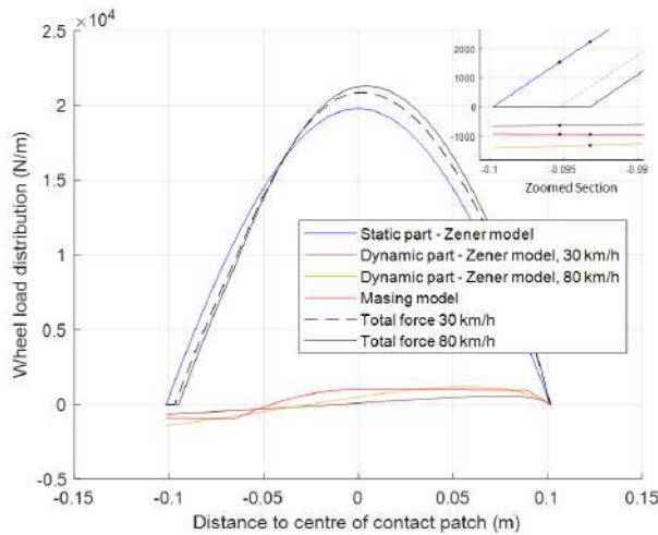
Figure 12 Modelled F_Z distribution for the cold class B tyre, with the speed dependant part of the model at two different speeds. A closeup of the lower left part of the graph is shown in the inset (see online version for colours)
