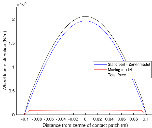
Figure 9 Contribution to static load for the cold class B tyre from the different parts of the model (see online version for colours)
