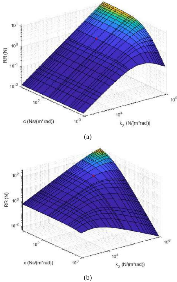
Figure 11 Rolling resistance modelled with the Zener model using different k_2 and c – values for the cold class B tyre. The red point shows the values used in the model: (a) simulated test speed 1.7 km/h and (b) simulated test speed 80 km/h (see online version for colours)
