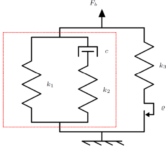
Figure 3 The bristle model built up by the Zener model with the parameters k_1 , k_2 and c , marked by a red frame, and the Masing model with the parameters \varrho and k_3 (see online version for colours)
