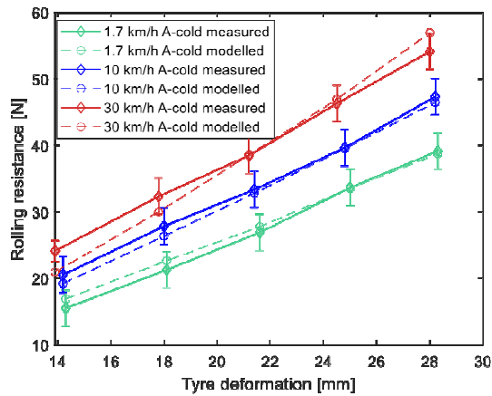
Figure 7 The measured and modelled rolling resistance against deformation for the three studied cases. The error bars indicate the measurement uncertainties: (a) cold class A tyre; (b) cold class B tyre and (c) warm class B tyre (see online version for colours)
